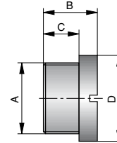
Dimensions Type: D1K Port size G1/8–G3/8
