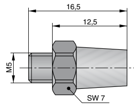
Dimensions Type: 50030 Port size M5
