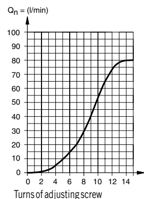
Flow characteristics Type: DV-M5
