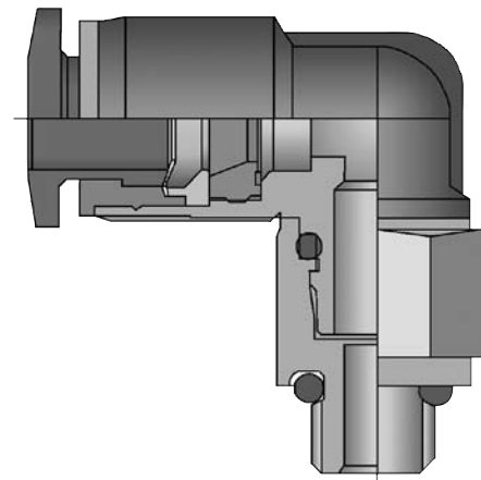
Elbow adaptor
