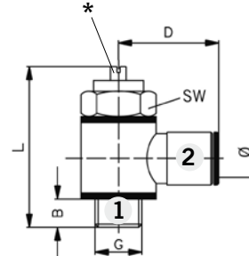
Screw-in throttle check valves Type: SEDRV-....A
