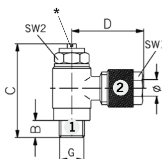
Screw-in throttle check valves Type: EDRV-....A
